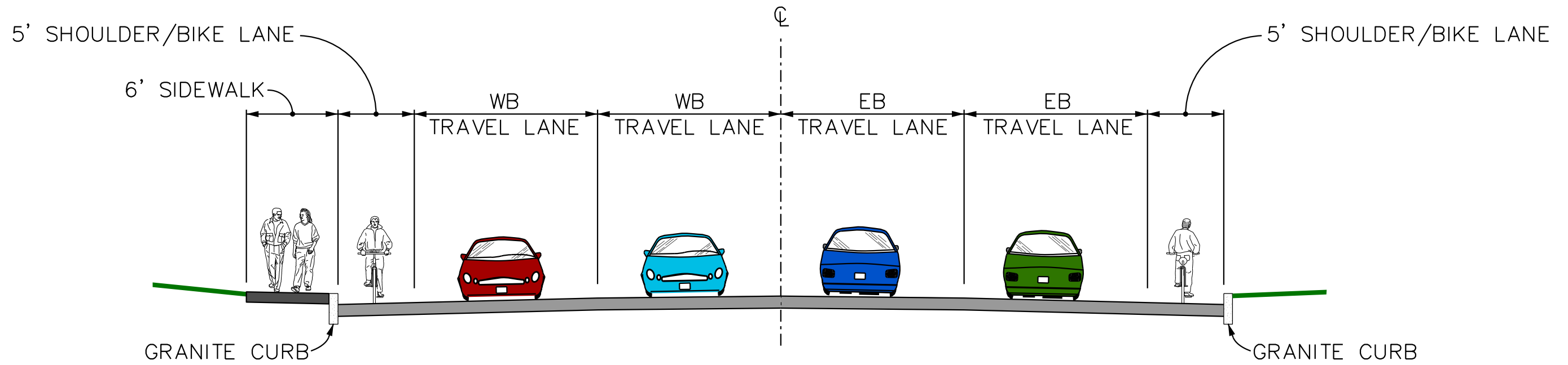
CONNECTOR ROAD - TYPICAL SECTION
